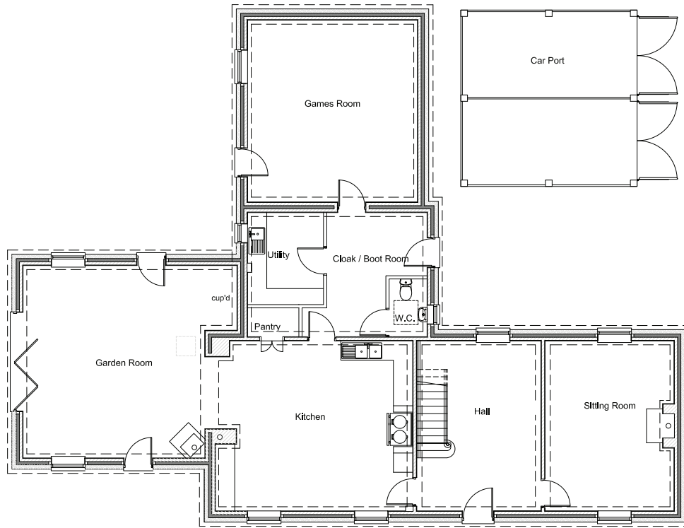
PLANS @ 1:50 (A1) Ground Floor
